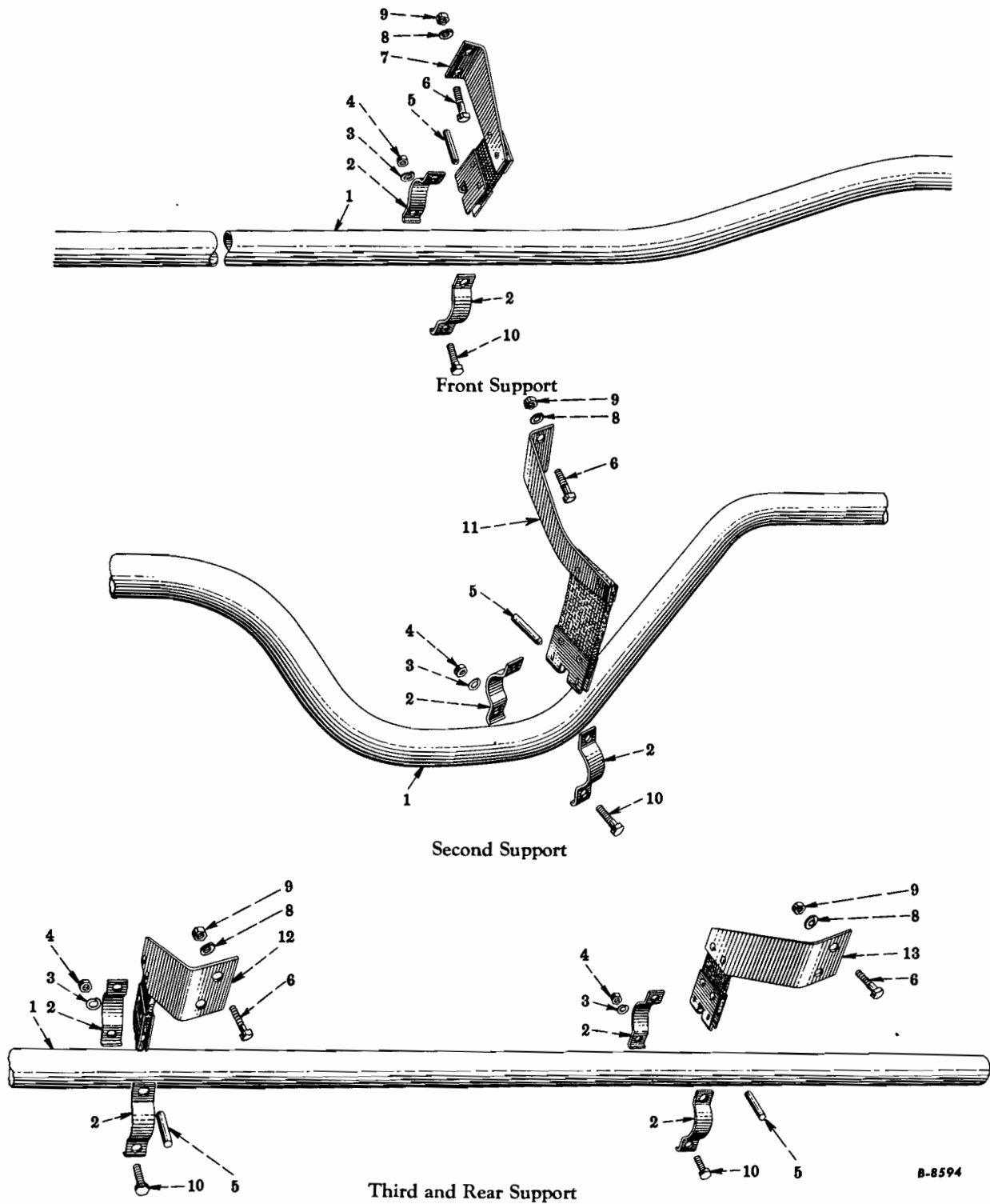
FIG. 07-7 - LONG TAIL PIPE (Code 0701) (R-160, R-163 With 190, 208" W.B.)
