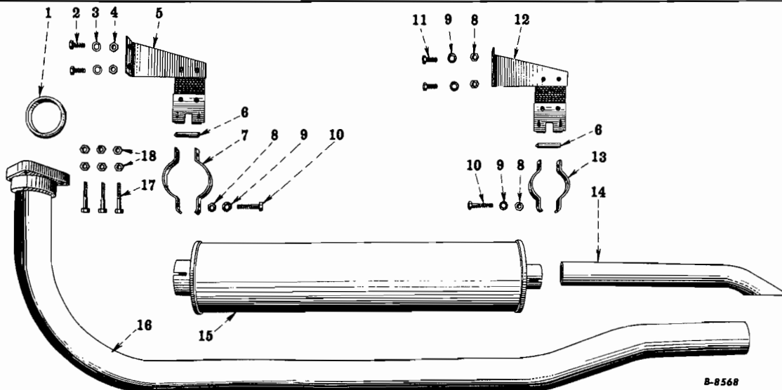
FIG. 07-2 - MUFFLER AND EXHAUST PIPE (with Short Tail Pipe)
